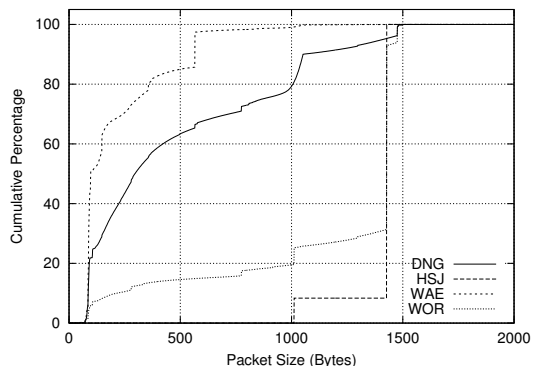
Fig. 6. Cumulative multicast packet size histograms (20:50 EDT July 2, 2001 to 20:50 EDT July 30, 2001)
